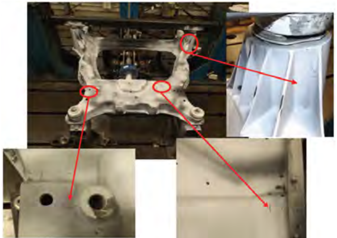
Figure 9: roll restrictor test cracks - CF subframes
