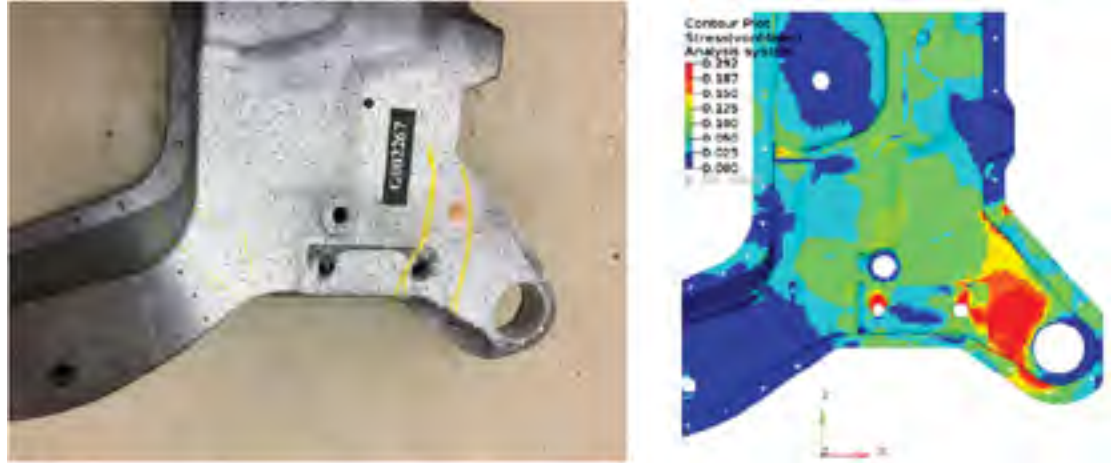
Figure 31: Strength test – control arm rear joint loading CAE failure location
