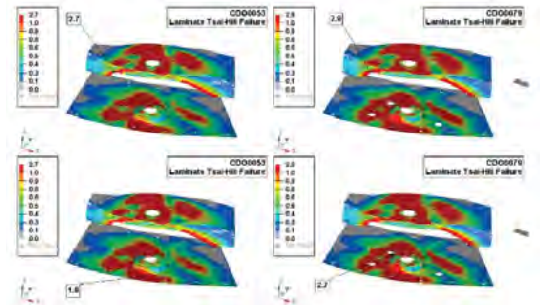
Figure 5: control arm front joint laminate surfaces
