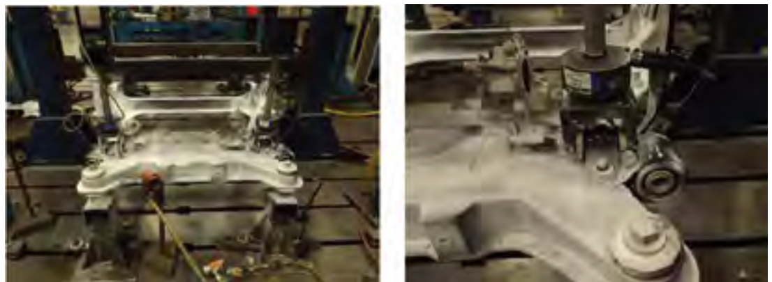
Figure 13: stabilizer bar test setup
